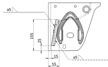
Area of lateral support including the weld
