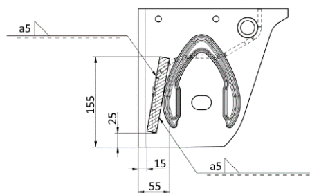
Area of lateral support including the weld
