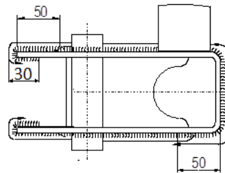
5.5 tonne / 7 tonne air suspension bracket with C-profile
