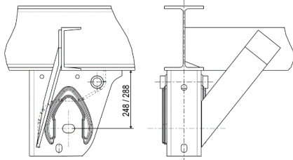
Suggested lateral support
