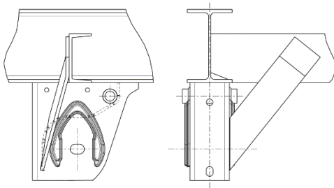
Suggested lateral support
