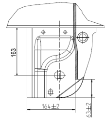
Area of lateral support including the weld
