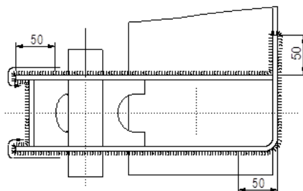
9 tonne air suspension bracket with C-profile
