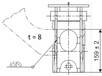
Suggested lateral support
