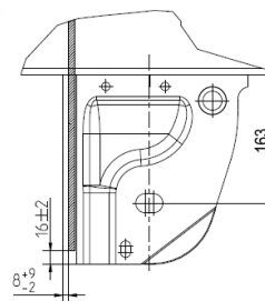
Area of lateral support including the weld
